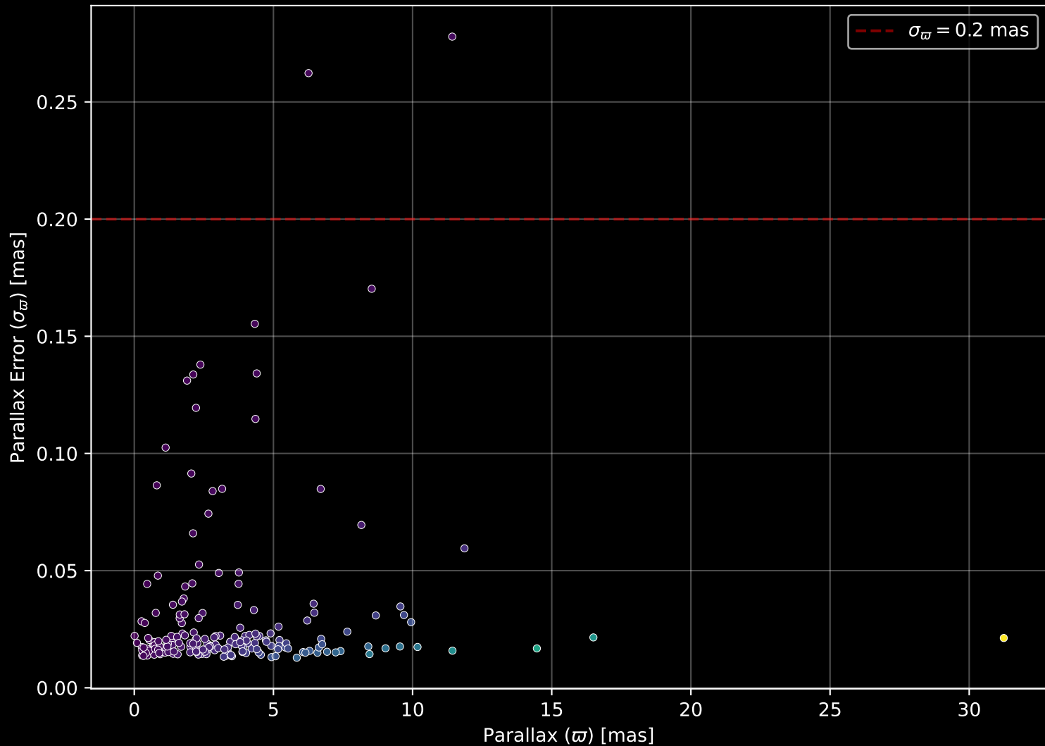
APOGEE DR17 Field: [180+33_MGA] Parallax Quality (n= 196)
