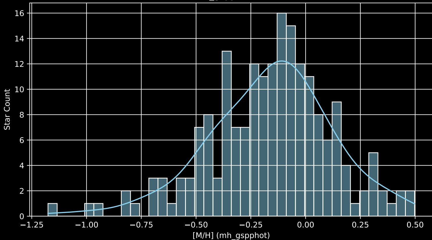
APOGEE DR17 Field: [180+33_MGA [M/H] (mh_gspphot) (n= 195)
