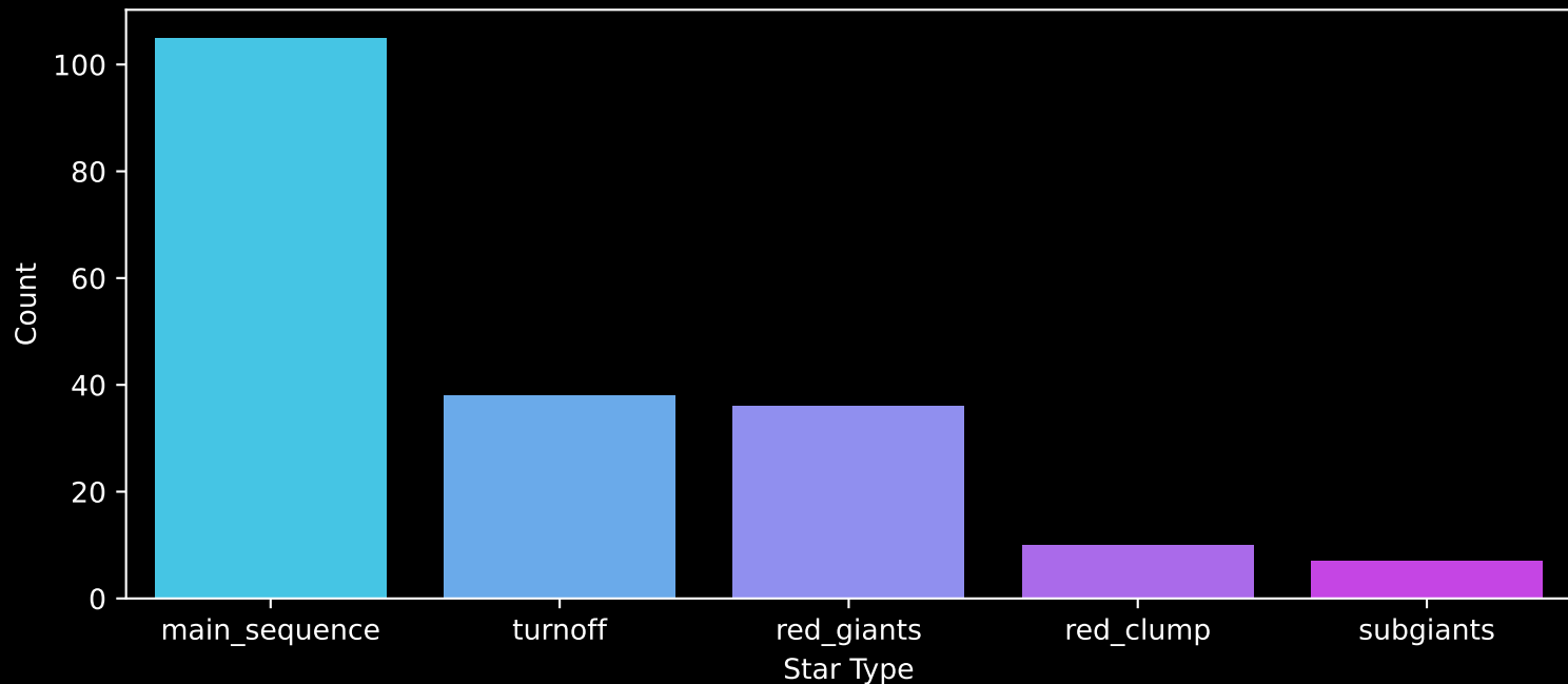
APOGEE DR17 Field: [180+33_MGA] Count plot of Star Type
