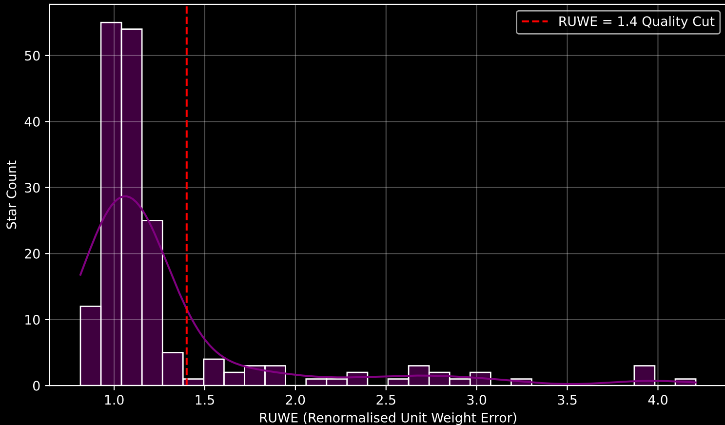
GAPOGEE DR17 Field [180+33_MGA] RUWE Distribution (n= 182)
