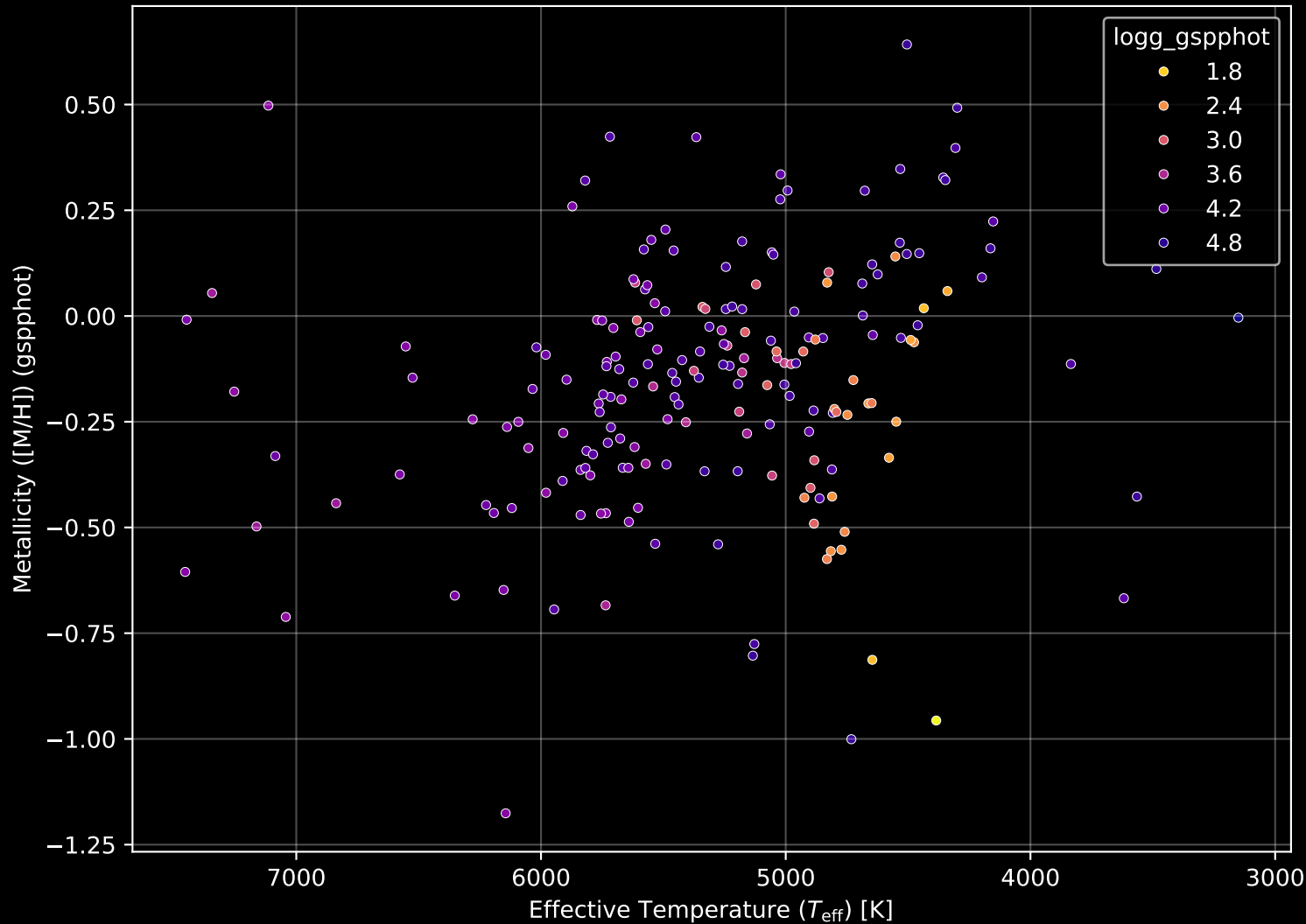
APOGEE DR17 Field: [180+33_MGA] Stellar Population Parameters (n= 196)
