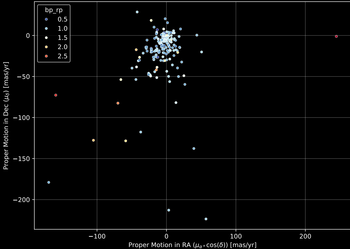
APOGEE DR17 Field: [180+33_MGA] Proper Motion Diagram (n= 196)
