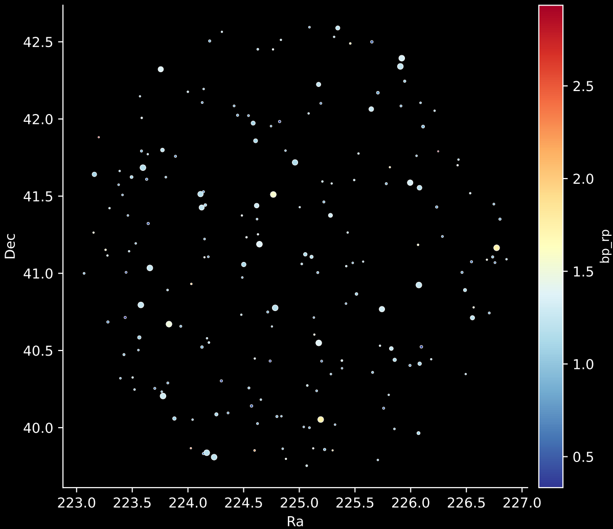
APOGEE DR17 Field: [180+33_MGA] Stars: 196
