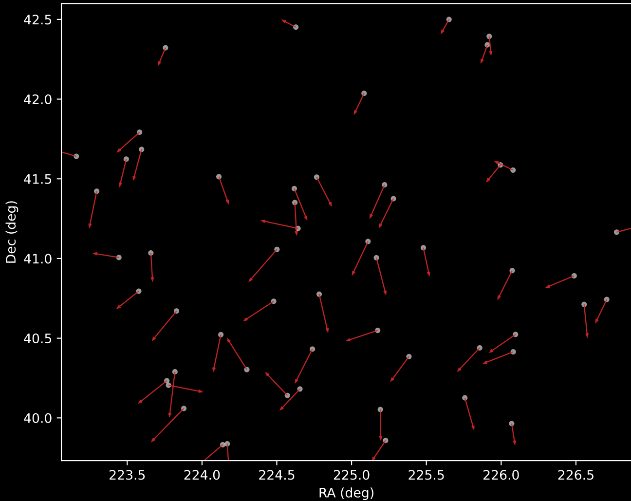
APOGEE DR17 Cluster 6 Proper Motion Vectors (n=55)
